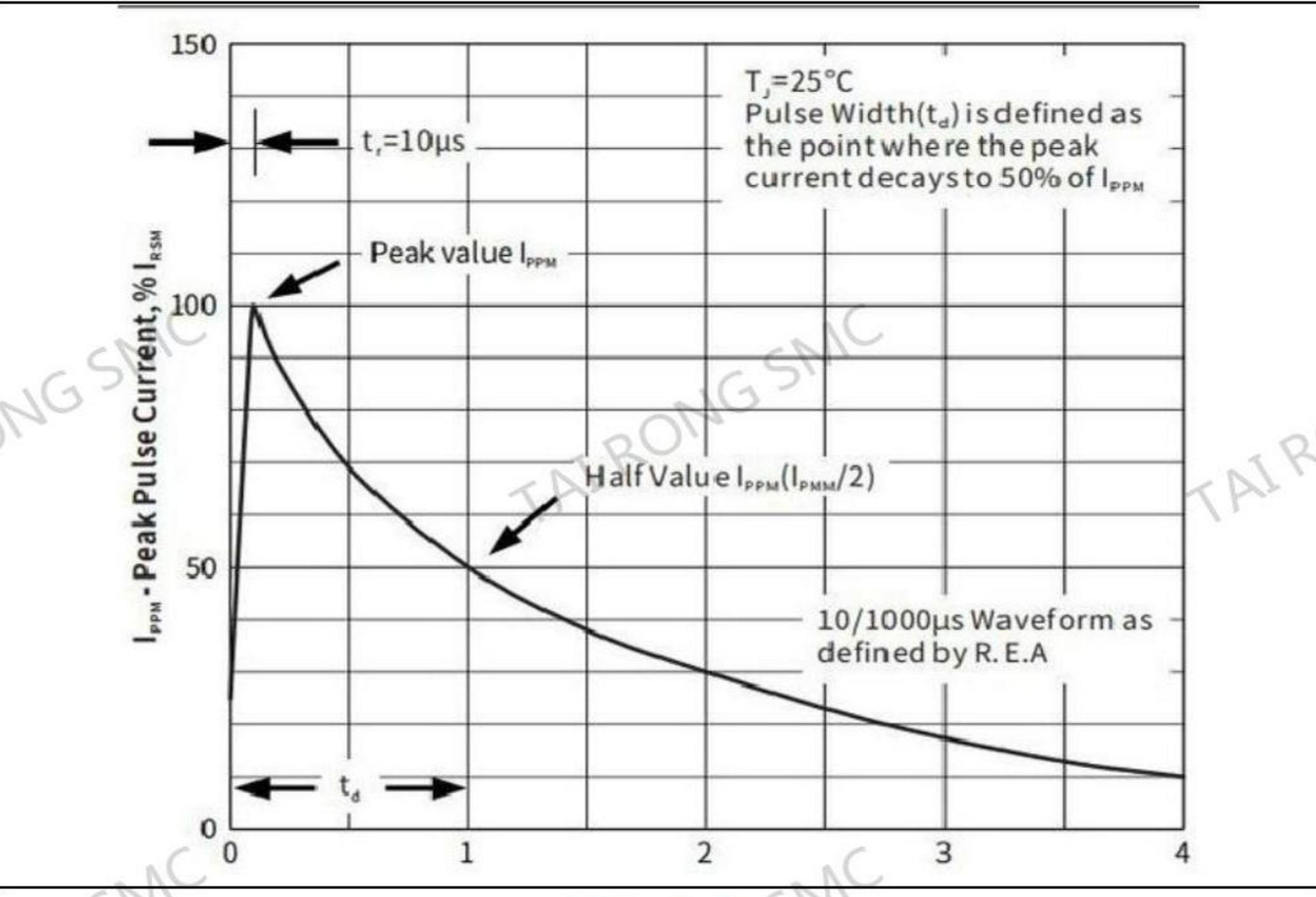
Fig.3 Pulse Waveform
