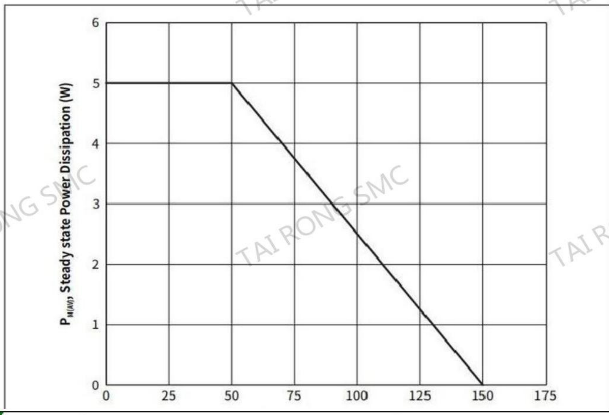
Fig.5 Steady State Power Dissipation Derating Curve
