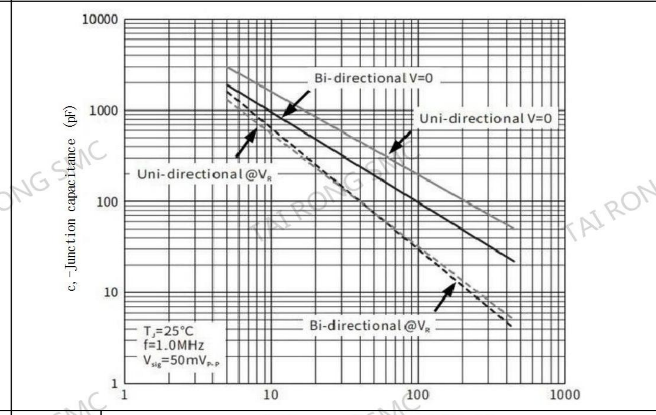
Fig.4 Typical Junction Capacitance
