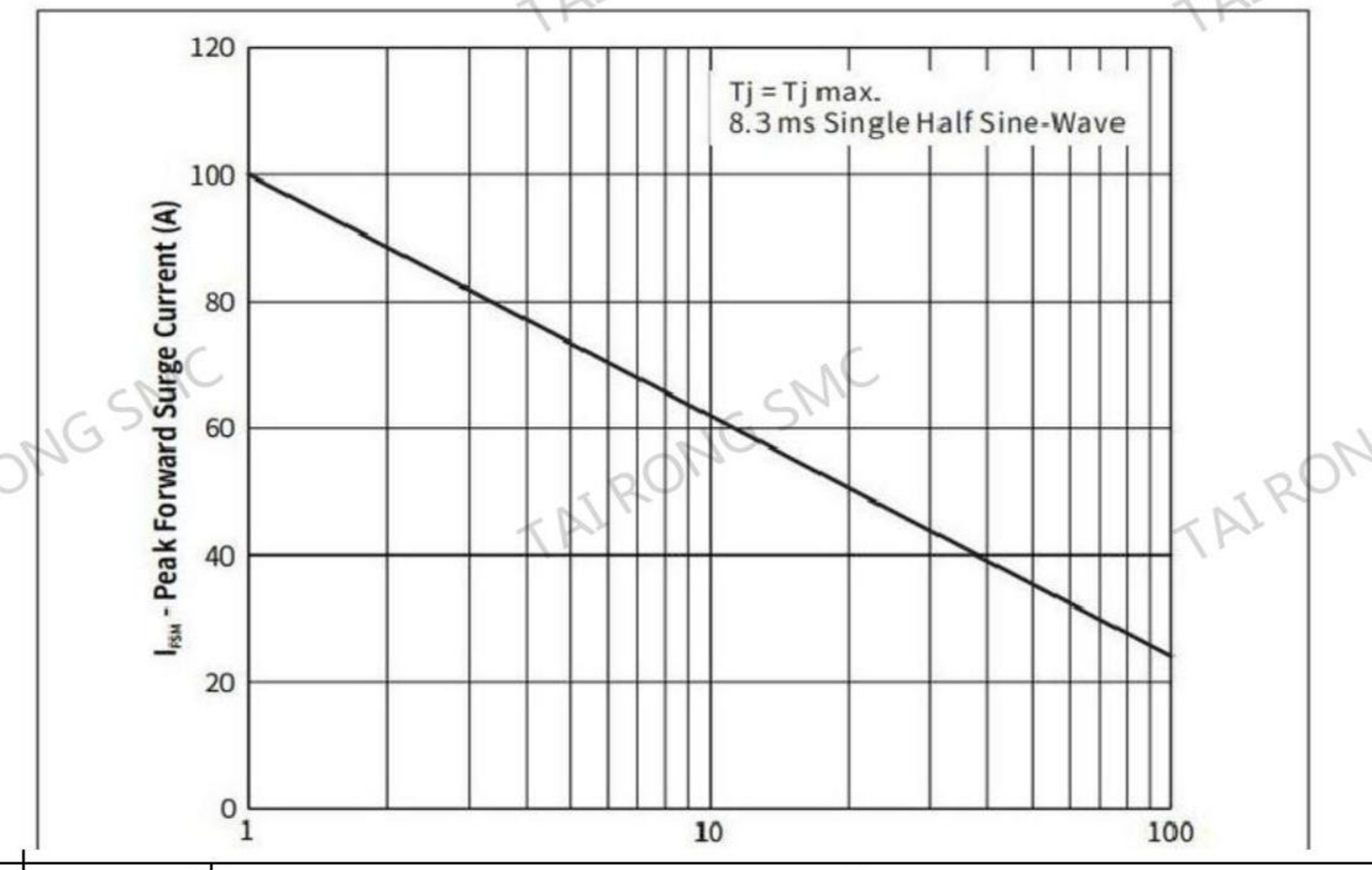
Fig.6 Maximum Non-Repetitive Forward Surge Current Uni-Directional Only
