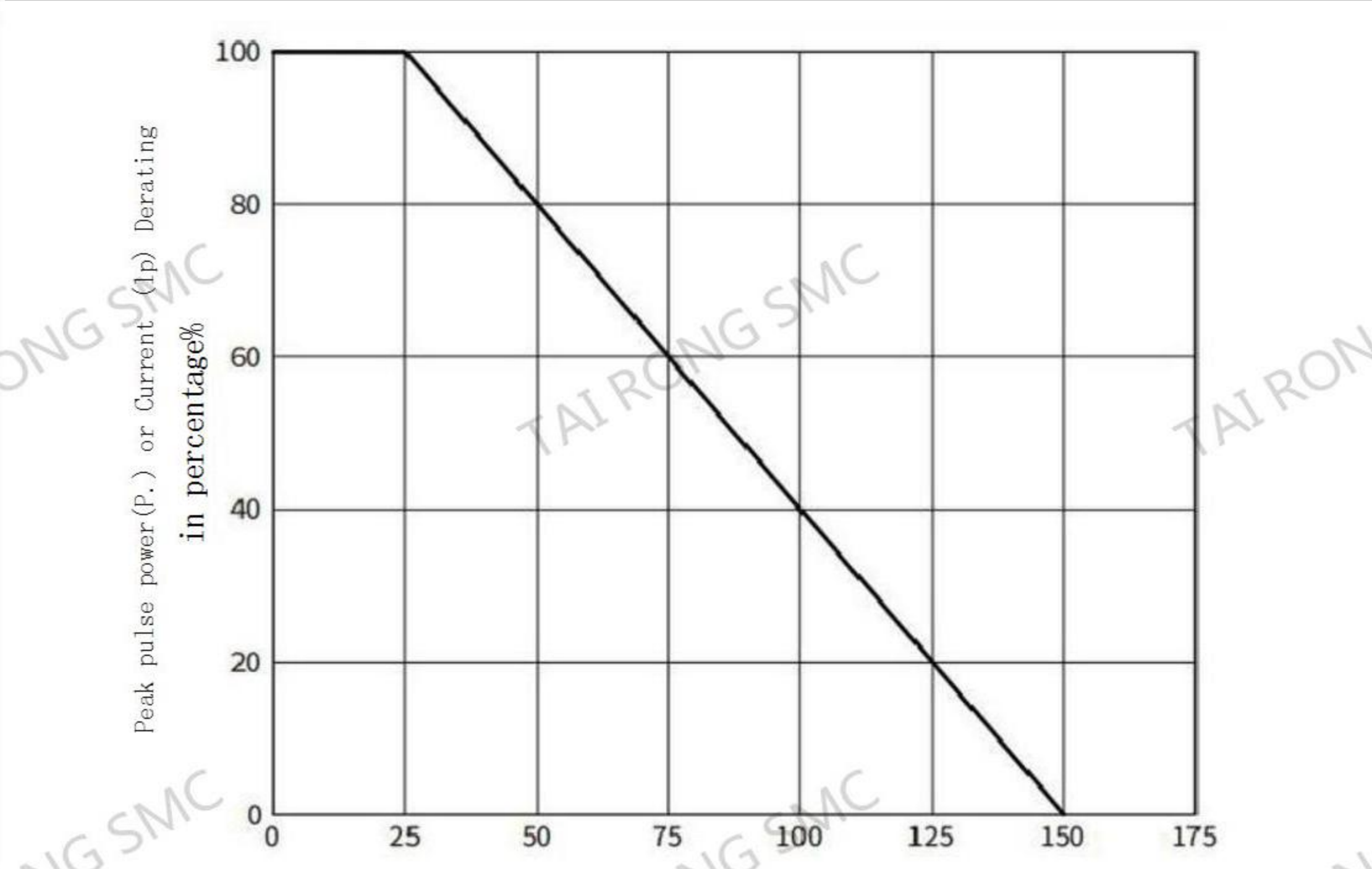
Fig.2 Pulse Derating Curve
