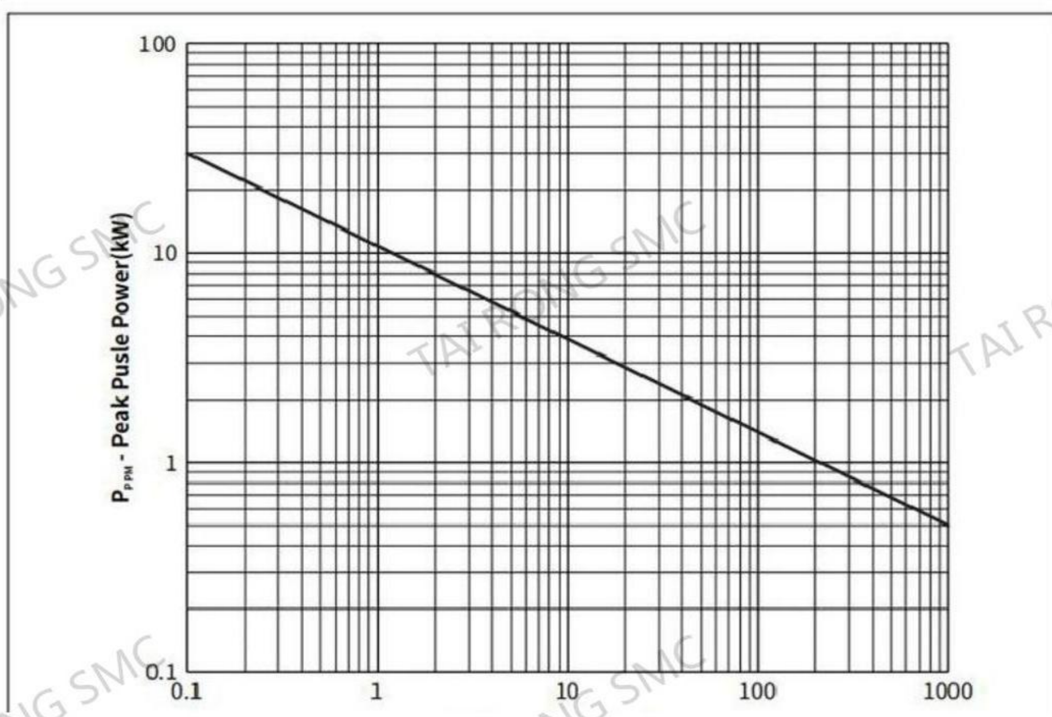
Fig.1 Peak Pulse Power Rating Curve
