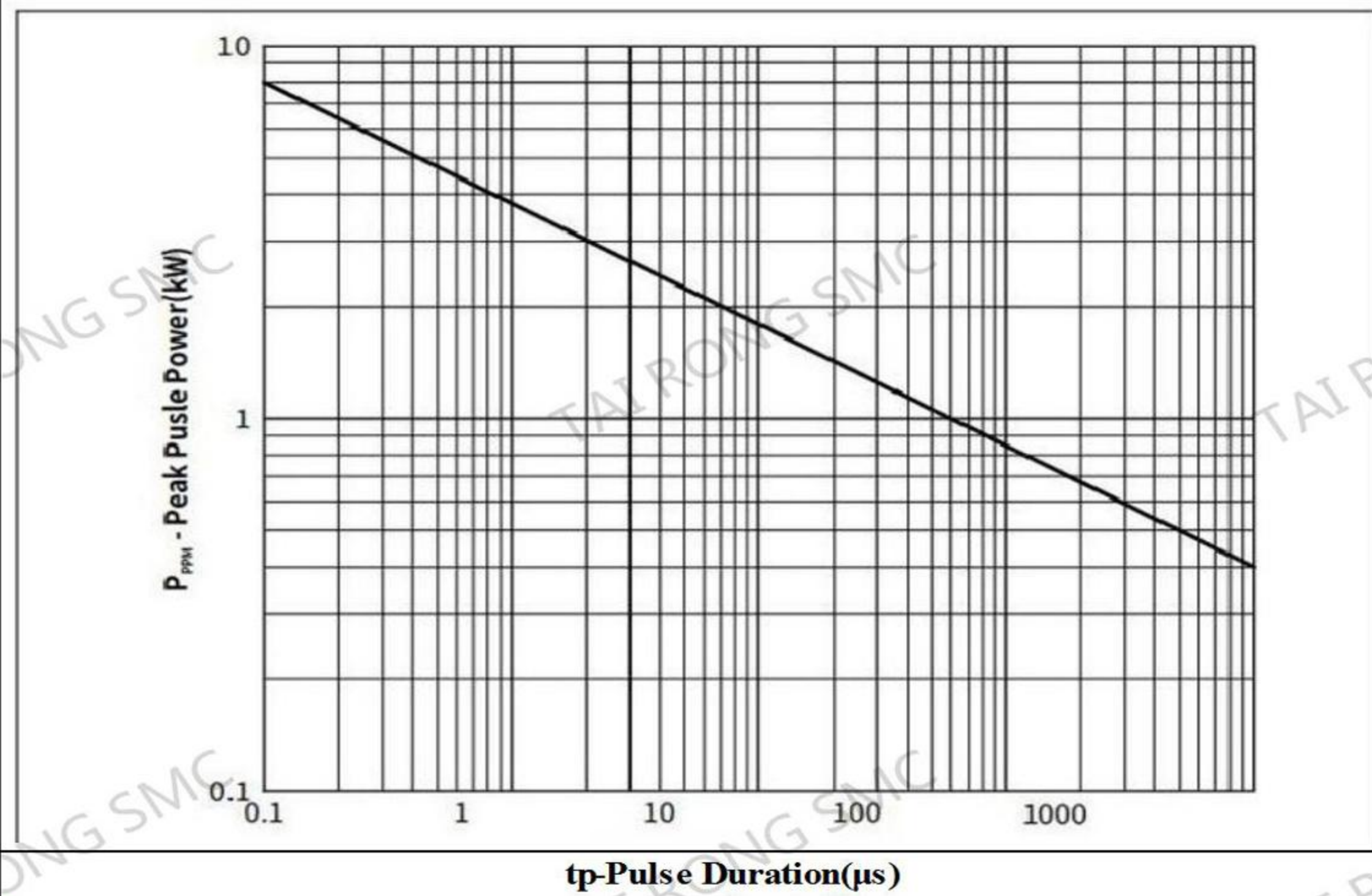
Fig.1 Peak Pulse Power Rating Curve
