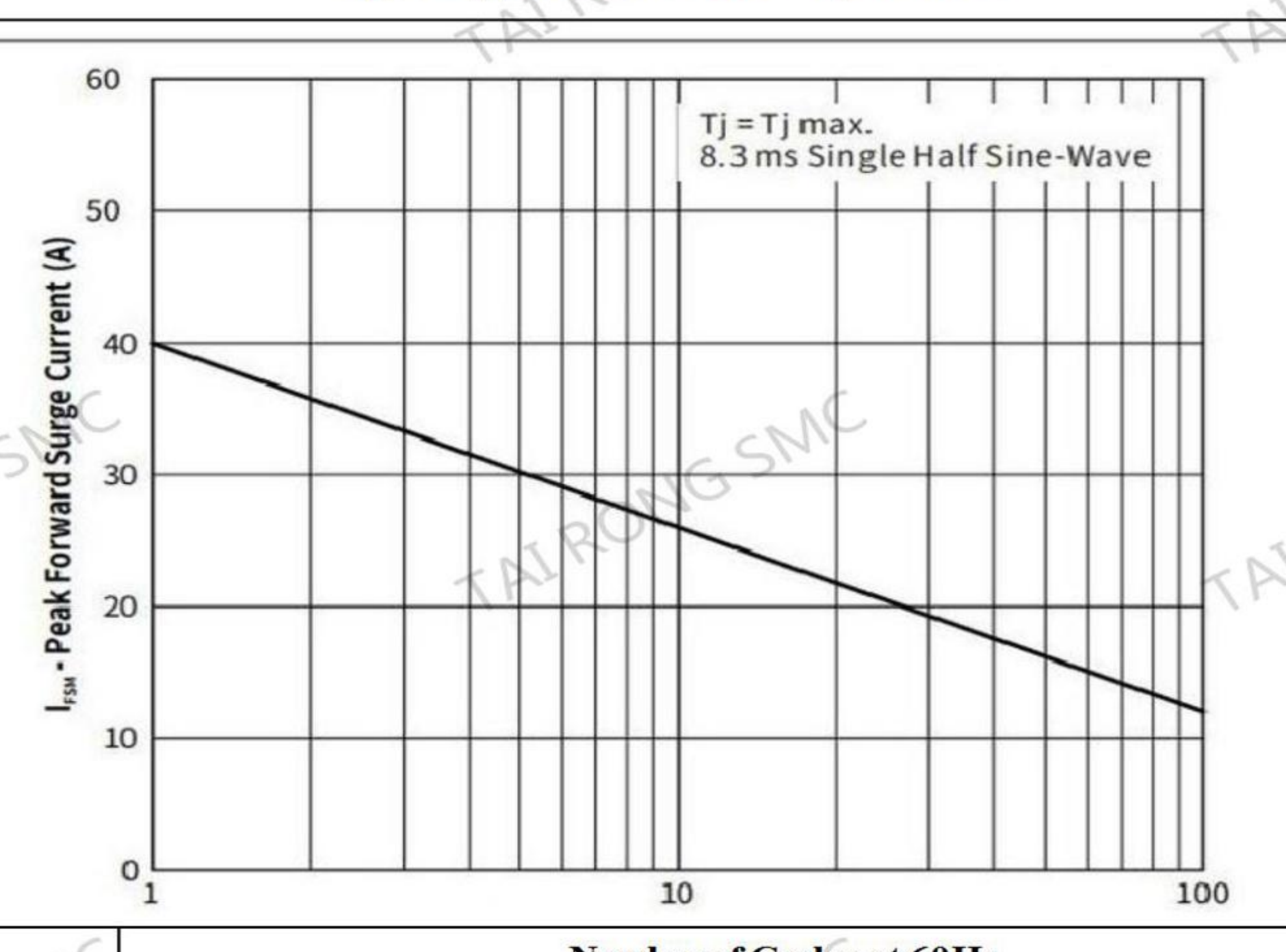
Fig.6 Maximum Non-Repetitive Forward Surge Current Uni-Directional Only
