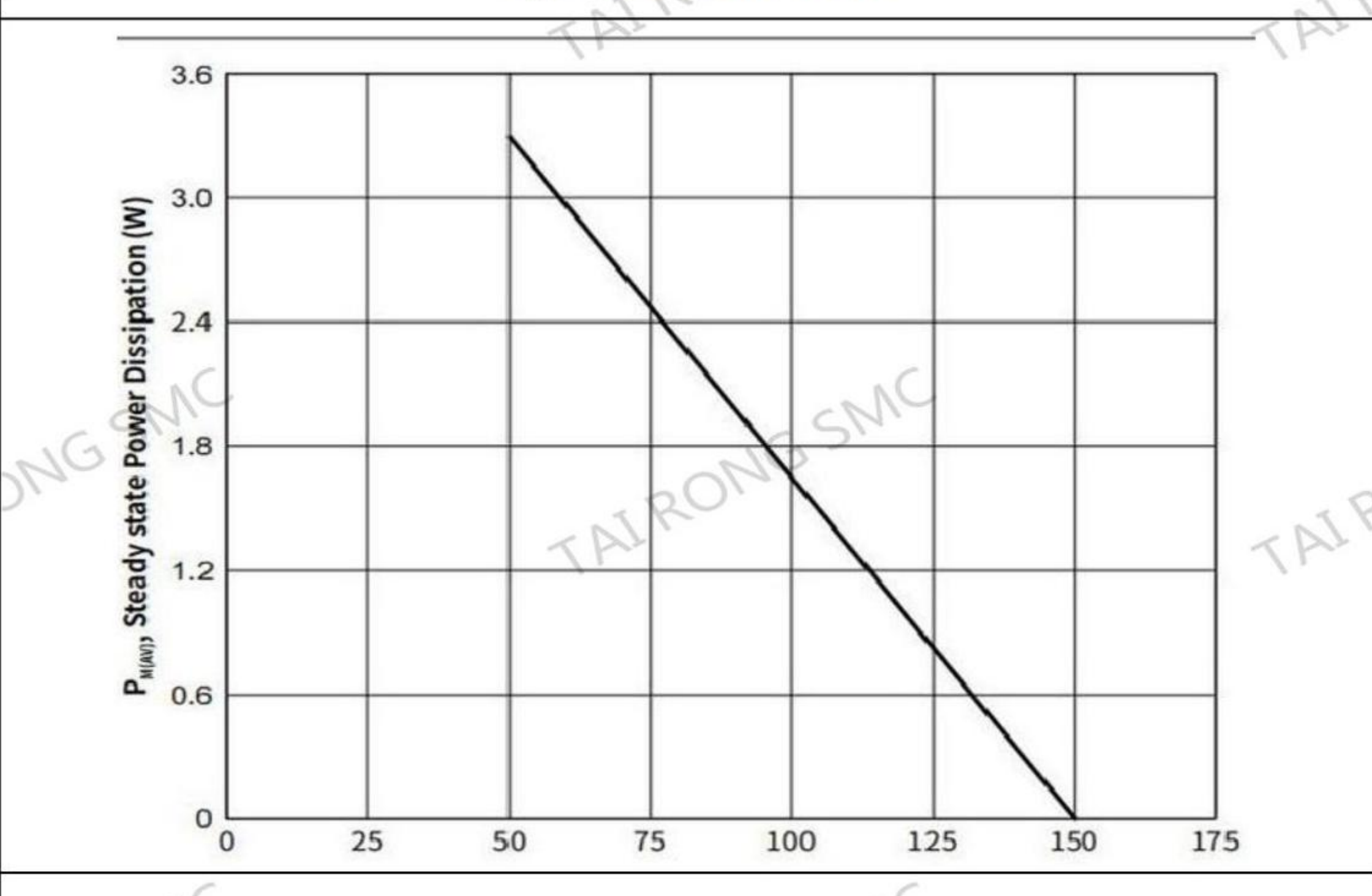
Fig.5 Steady State Power Dissipation Derating Curve
