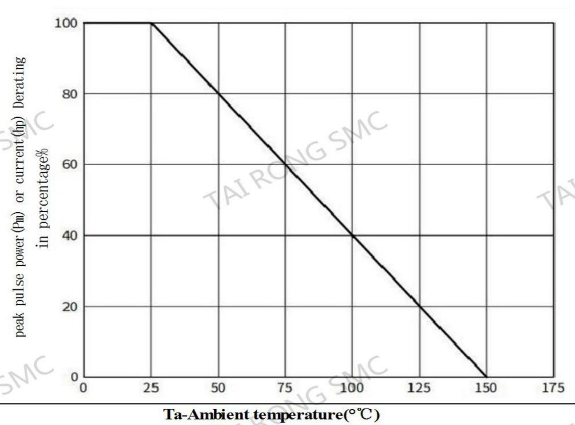
Fig.2 Pulse Derating Curve
