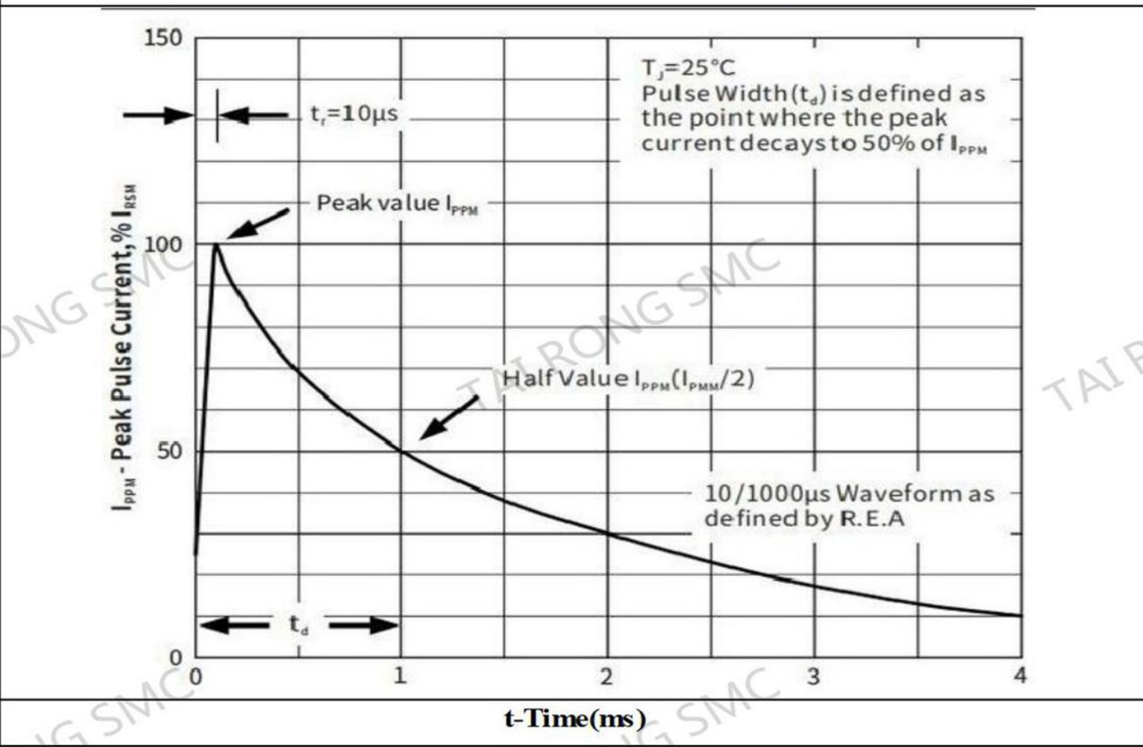
Fig.3 Pulse Waveform
